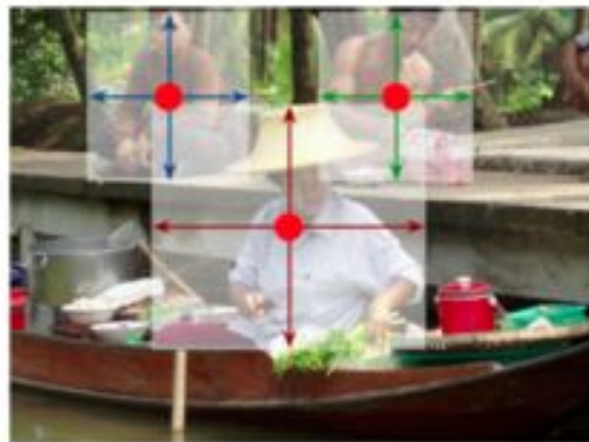
Figure 2: We model an object as the center point of its bounding box. The bounding box size and other object properties are inferred from the keypoint feature at the center. Best viewed in color.
